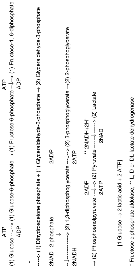
Figure 11.2 Homolactic fermentation of hexoses through the EMP pathway.
